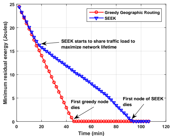
Figure 18: Maximum energy consumed by a node
