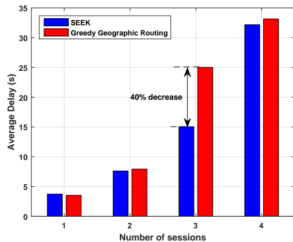
Figure 23: Average Delay vs No. of sessions
