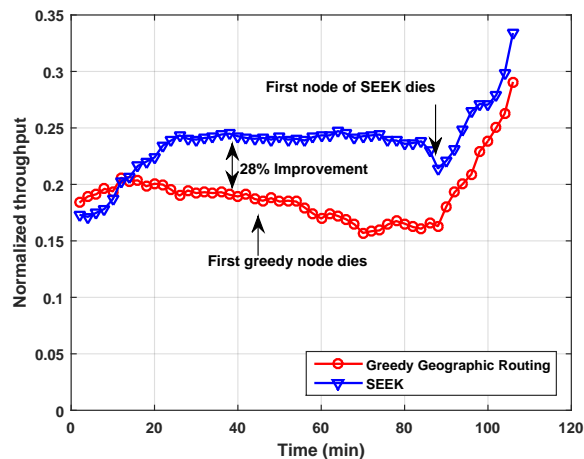
Figure 19: Normalized throughput of the network
