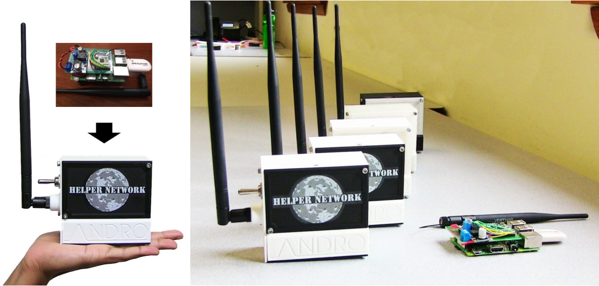
Figure 11: HELPER Prototype
