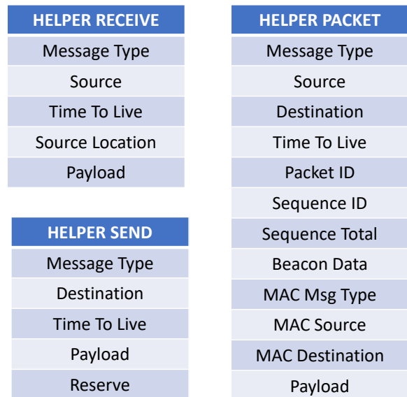
Figure 8: Packet formats
