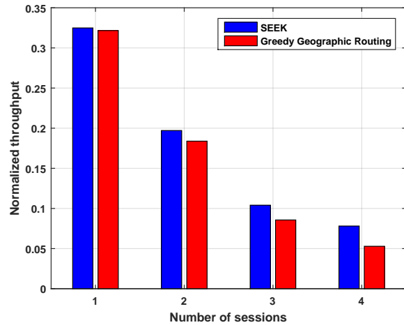
Figure 21: Normalized throughput vs No. of sessions
