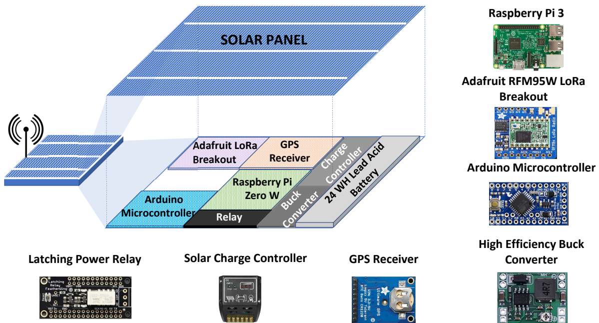
Figure 2: Static HELPER Design
