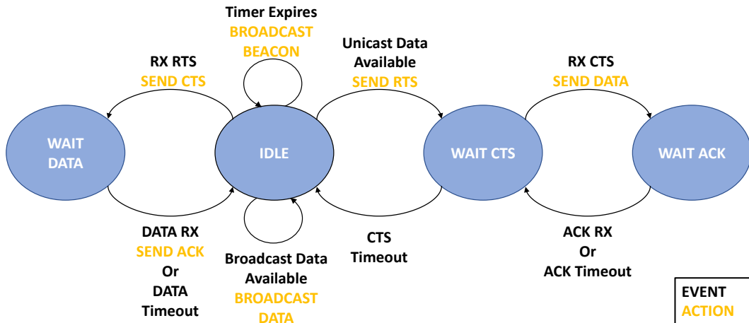
Figure 6: FSM of the MAC protocol
