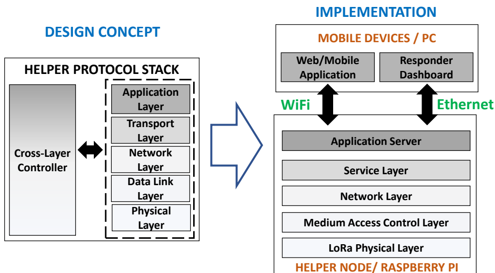
Figure 5: HELPER's cross-layer Protocol stack design and implementation
