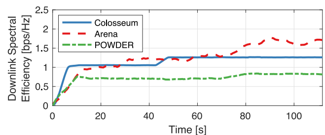
Figure 17: Downlink spectral efficiency of SCOPE ported on three different testbeds: Colosseum, Arena and POWDER.
