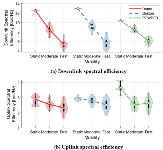
Figure 8: Spectral efficiency in the dynamic scenarios.
