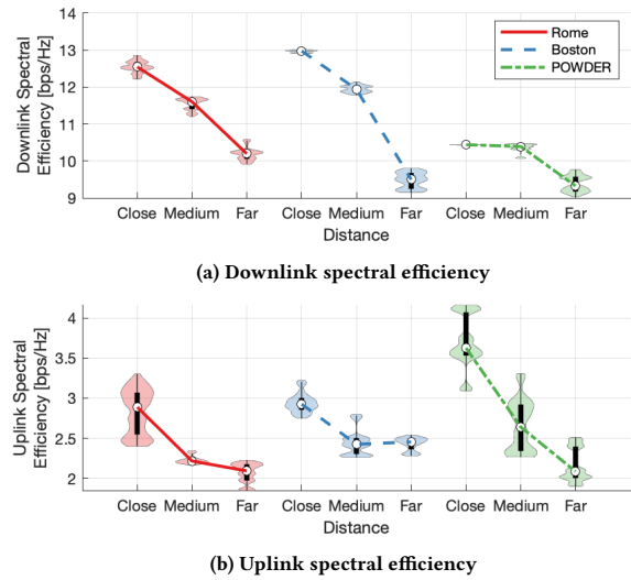
Figure 7: Spectral efficiency in the static scenarios.
