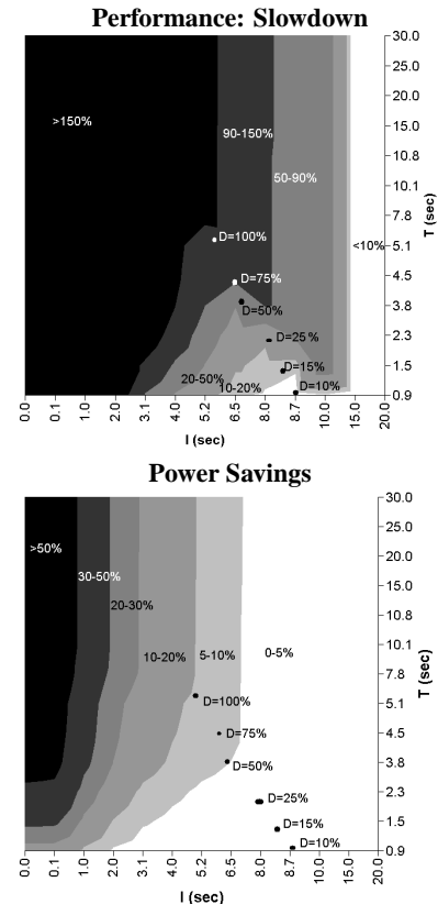
Figure 1: Performance slowdown (top) and power savings potential (bottom) in a test case (a disk in a file server).
