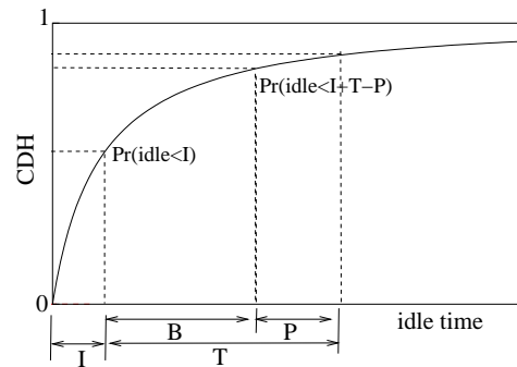
Figure 2: Estimation of the amount of time B that the disk stays in the idle mode with penalty P which starts after I units of idle time have elapsed and ends T time units later.
