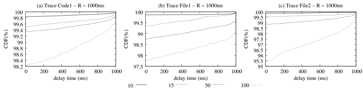
Figure 5: Distribution of delays in user requests attributed to power savings under level 4 for slowdown targets equal to 10, 15, 50, and 100.
