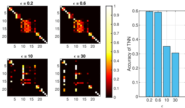
Figure 3: Confusion matrix of MC TNN under the AWJ-U attack in low SNR regime for different \epsilon values. Figure 4: Accuracy of MC TNN in Fig. 3 (originally 60%).
