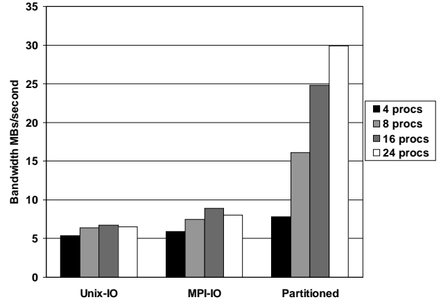
Figure 6: SPEChpc write bandwidth in MBs/second.
