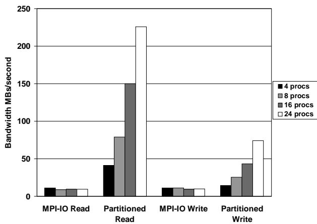
Figure 8: Perf read and write bandwidth in MBs/second.
