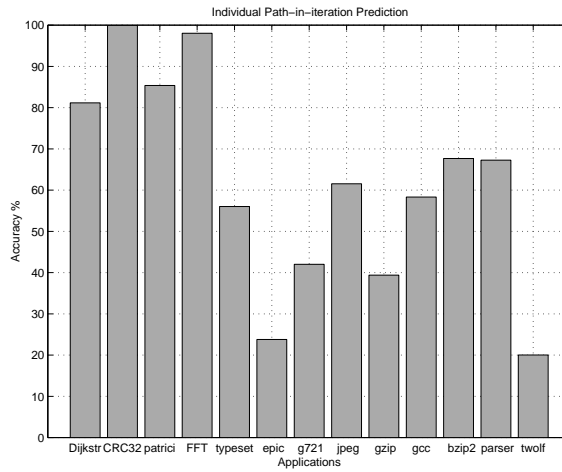
Figure 5. Prediction of path-in-iteration per loop iteration.
