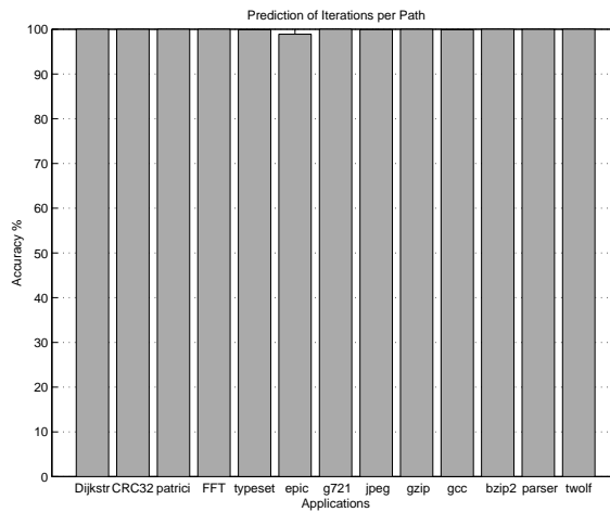
Figure 6. Prediction of number of iterations for path-in-iteration.
