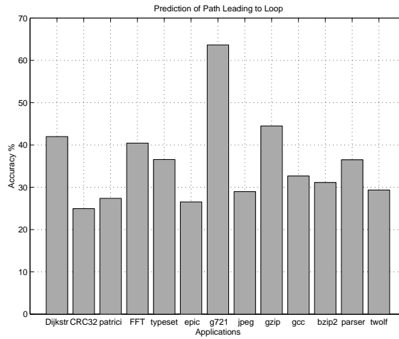
Figure 3. Prediction of entering the loop using the path-to-loop.
