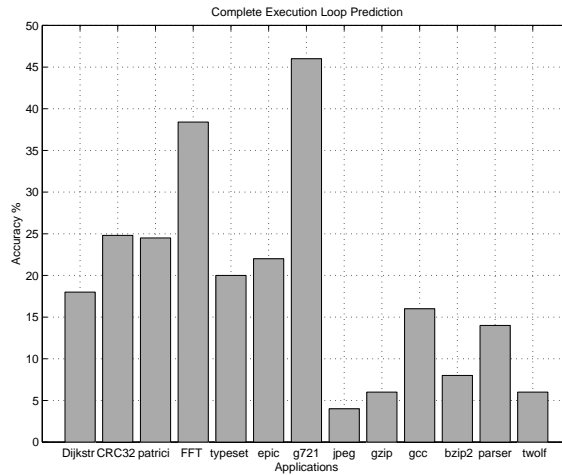
Figure 7. Loop Execution Prediction.
