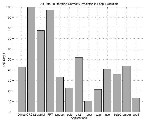
Figure 4. Prediction of path-in-iteration per loop visit.
