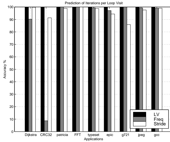
Figure 1. Prediction accuracy of the number of iterations per loop visit, comparing 3 different predictors.
