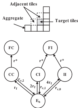
Figure 3. Kinetic trap model for double bonding under constant monomer concentration: target tile mode
