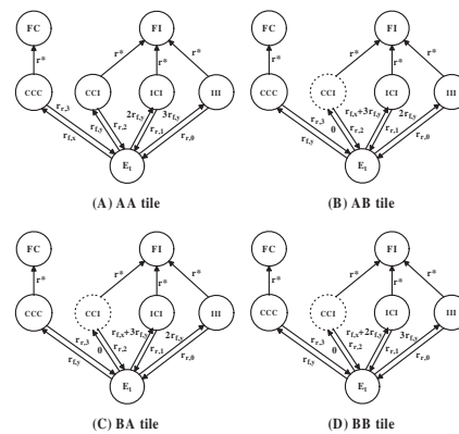
Figure 7. Kinetic trap model for triple bonding under non-constant monomer concentration: the dotted circle denotes a dummy state used for readability
