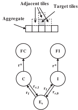
Figure 2. Kinetic trap model for single bonding under constant monomer concentration: target tile mode
