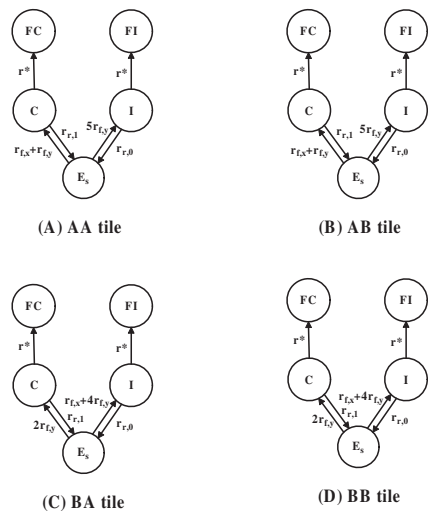
Figure 5. Kinetic trap model for single bonding under non-constant monomer concentration
