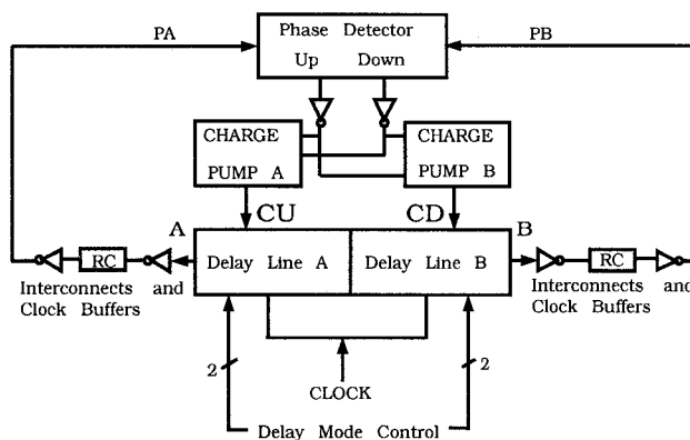
Fig.1 Block level structure of the DLL circuit.
