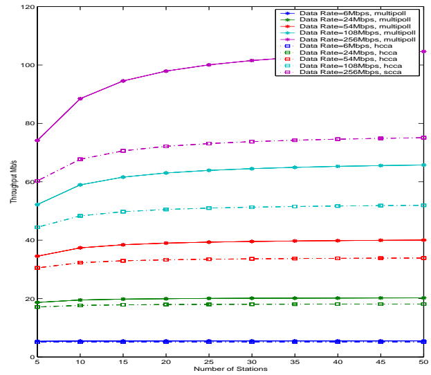
Fig. 4. Throughput Comparison of Proposed Multi-Poll over 802.11e
