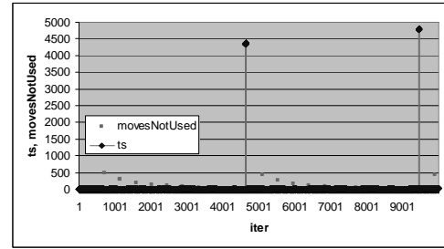
(a) SC-Tabu behavior on a QAP - random uniform distribution problem
