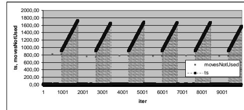
(b) SC-Tabu behavior on a QAP - real life like problem
