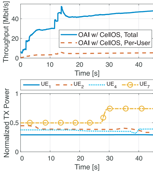
Fig. 9. Sum-log-rate maximization in the low interference scenario on the OAI-based prototype w/ CellOS.
