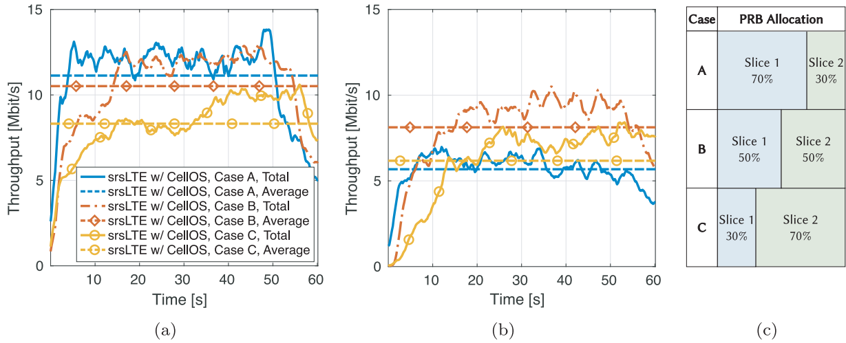
Fig. 11. Optimization of different control programs on different slices on the srsLTE-based prototype instantiated on the Arena testbed [32]: (a) Throughput of Slice 1 ( \max(\text{rate}) ); (b) throughput of Slice 2 ( \min(\text{power}) ); (c) PRB allocation.
