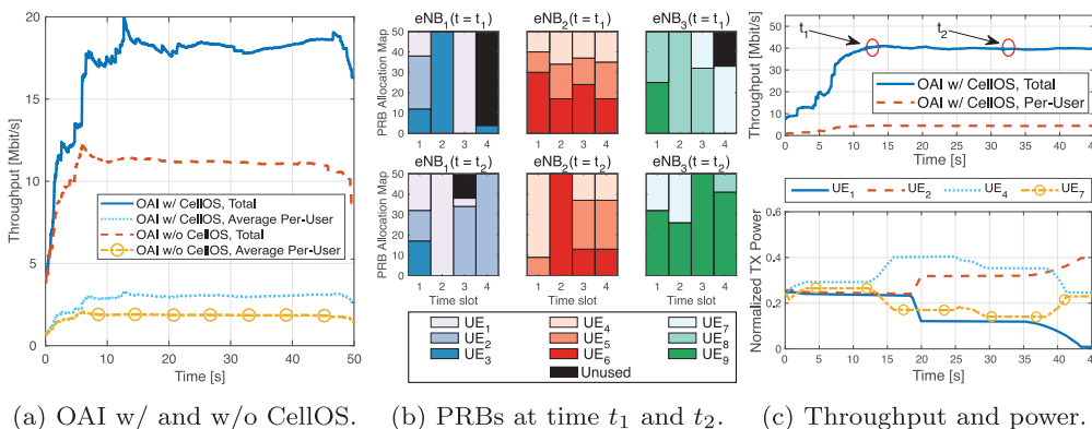
Fig. 6. Throughput maximization in the high interference scenario on the OAI-based prototype.
