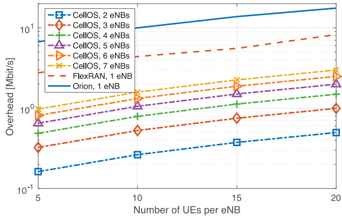
Fig. 14. Signaling overhead: CellIOS vs. FlexRAN [13, Figure 7] and Orion [44, Figure 13a].
