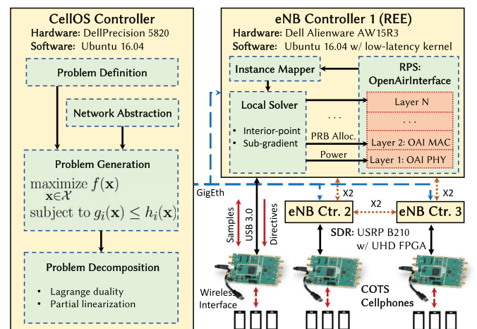
Fig. 4. OAI-based CellOS prototype.
