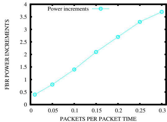
Figure 2: Number of FBR power increments.
