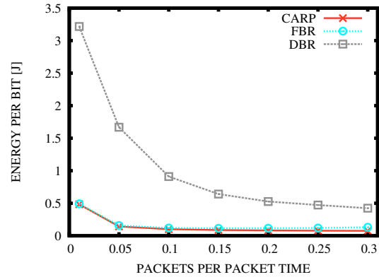
Figure 5: Energy consumption per bit: Case with idling.
