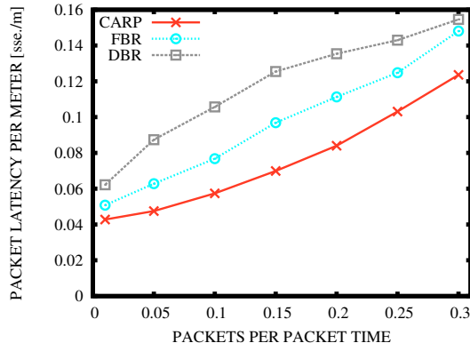
Figure 3: Latency per meter.
