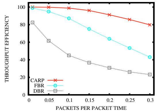
Figure 1: Throughput efficiency.
