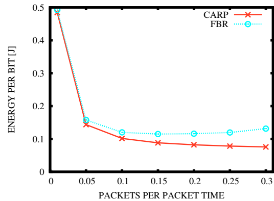
Figure 6: Energy consumption per bit: CARP and FBR (zoom).
