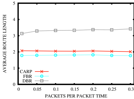
Figure 4: Route length.
