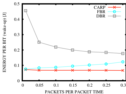
Figure 7: Energy consumption per bit: Case with “wake up modems.”
