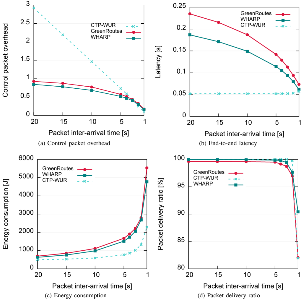
Fig. 4. Performance comparison of CTP-WUR, GREENROUTES and WHARP for increasing traffic.
