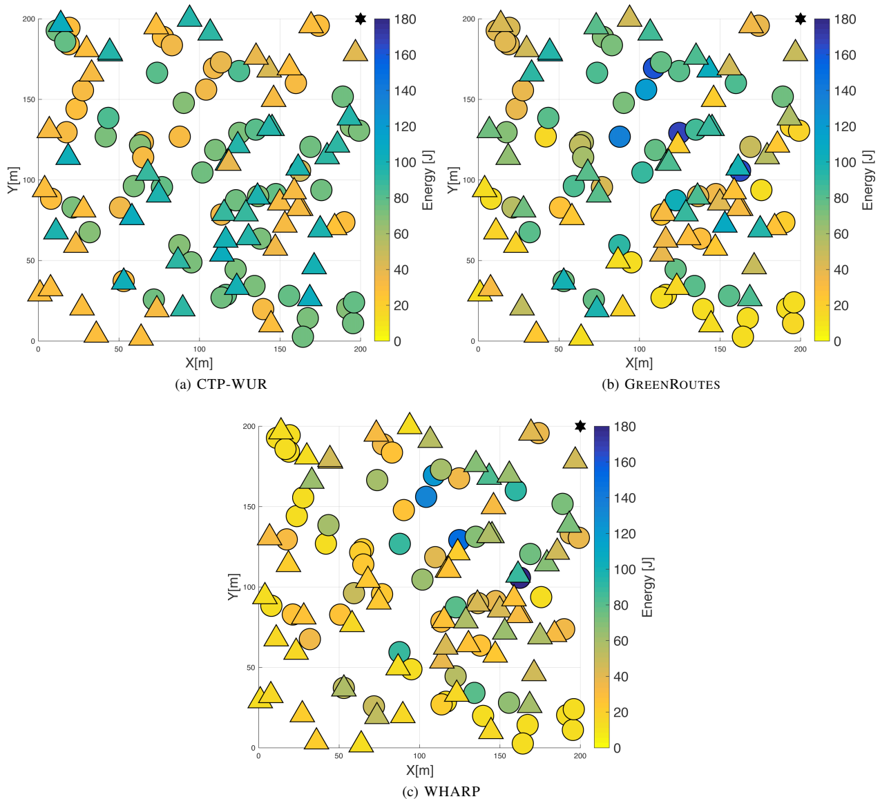
Fig. 6. Per node energy consumption in networks with medium/high traffic and heterogeneous energy harvesting sources.
