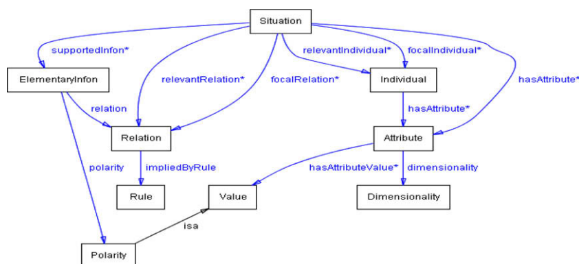
Fig. 4. Main classes and properties of STO.
