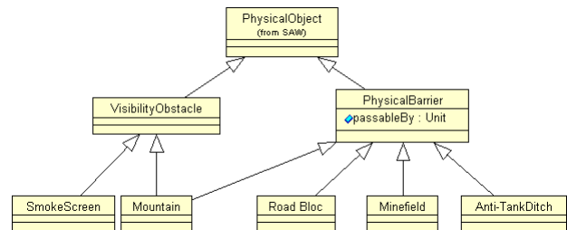
Figure 10. Battlefield Ontology - Obstacles
