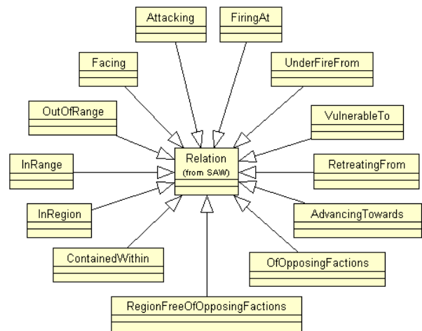
Figure 11. Battlefield Ontology – Relations
