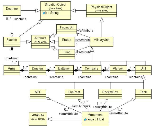
Figure 9. Battlefield Ontology – Military Units
