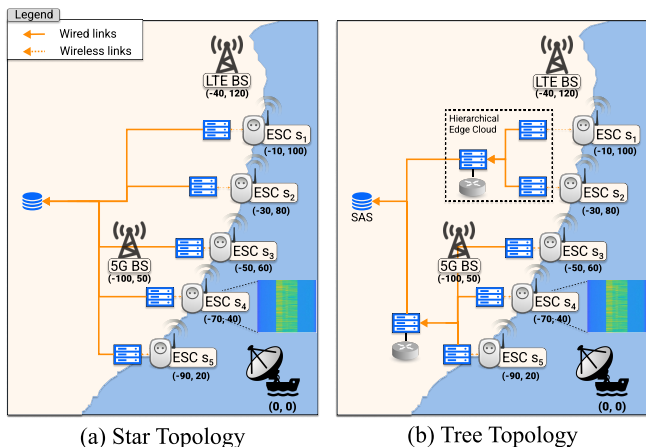
Fig. 5: A schematic of the deployment of CBRS case study using CaP framework. All distance units are in km. We only focus on the processing part of the deployment. During the deployment either of (1) Star or (2) Tree topology are used. We provide the comparative analysis between the two topologies in Table IV.
