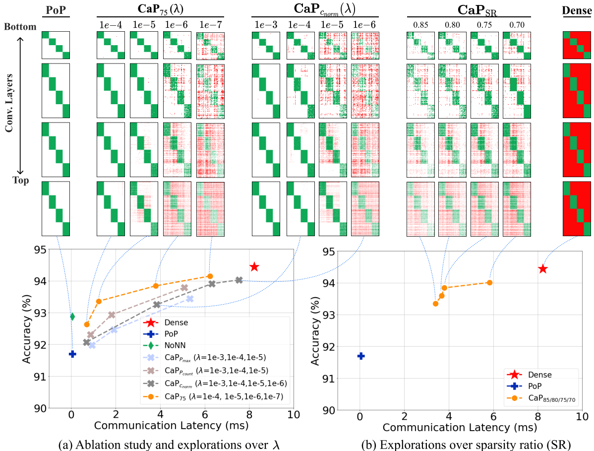
Fig. 4: We perform an ablation study over the (a) balancing parameter \lambda and (b) sparsity ratio (SR) on CIFAR-10 by ResNet-18 under a 4-device setting. In particular, we set \text{SR}=0.75 for all variants in (a) and set \lambda=1e-6 when exploring SR in (b). For reference purposes, we also include (a) a dense model, (b) a fully partitioned model PoP, and (c) NoNN. We show the trade-off between accuracy and communication latency. To visualize the partitioning, we further show the learned tensors on selected layers, from bottom (i.e., nearer to the inputs) to top, and color the weight tensor kernel-wise, resulting in a colored matrix with a size of P_l' \times P_l : each entry indicates the absolute sum over a kernel, colored by white for zeros, green for non-zeros within the same device, and red for parameters used in cross-device communications.
