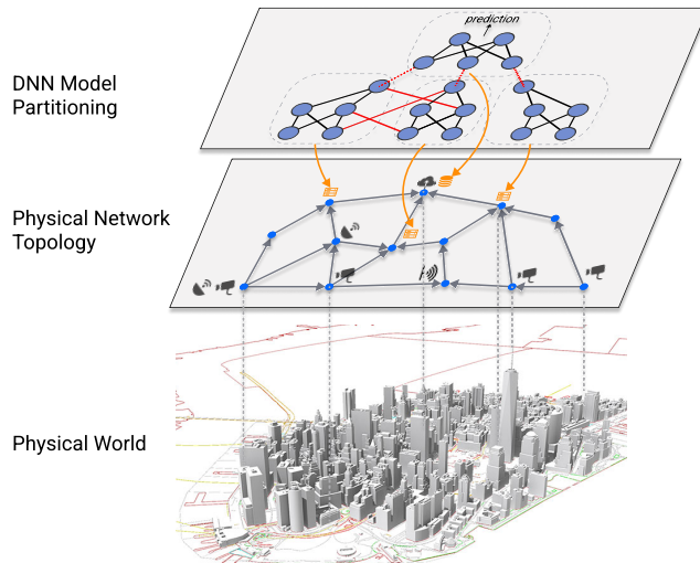
Fig. 1: Motivation of our CaP framework. We consider a smart city as a motivating scenario, involving a ubiquitous deployment of networked sensors at different locations across a large urban area. To reduce latency and accelerate computation, inference over a DNN is distributed across the network fabric. Using CaP, the DNN model can be partitioned into sub-networks, each of which is mapped to the physical network topology; our goal is to reduce latency while maintaining predictive performance.
