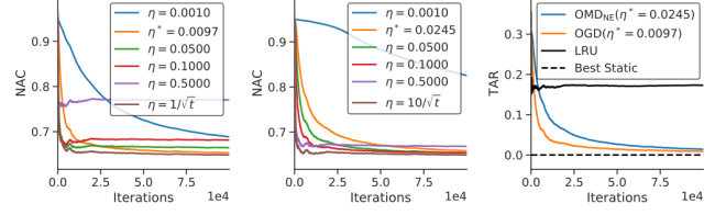
(a) NAC of OGD (b) NAC of \text{OMD}_{\text{NE}} (c) Time-Average Regret
