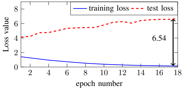
(a) Loss without data augmentation (DA)
