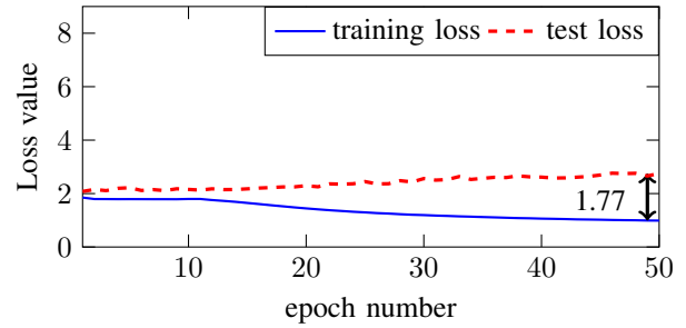
(b) Loss with data augmentation (DA)
