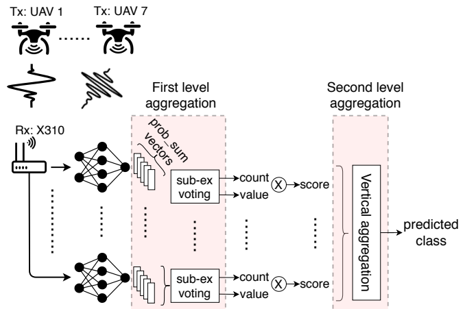
Figure 1: UAV classification using multi-classifier scheme with two levels of aggregation.
