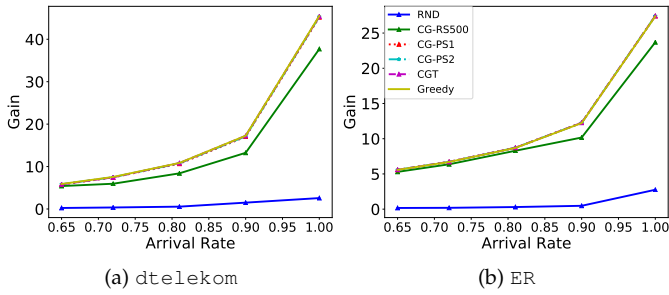
Fig. 7: Caching gain vs. arrival rate. As the arrival rate increases caching gains get larger.
