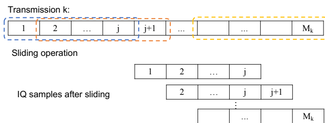
Figure 3. An illustration of generating slices from an arbitrary-length sequence. Given a time-series of length M_k , we create M_k - j + 1 subsequences of length j by sliding a window of length j over the larger sequence (or stream) of I/Q samples (with stride 1). This leads to inputs of a fixed length, but also enhances shift invariance. The (full) sequence can be classified by using a label aggregation method over its constituent slices.
