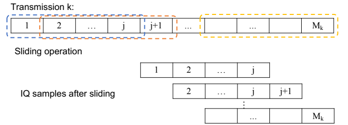
Figure 3. An illustration of generating slices from an arbitrary-length sequence. Given a time-series of length M_k , we create M_k - j + 1 subsequences of length j by sliding a window of length j over the larger sequence (or stream) of I/Q samples (with stride 1). This leads to inputs of a fixed length, but also enhances shift invariance. The (full) sequence can be classified by using a label aggregation method over its constituent slices.
