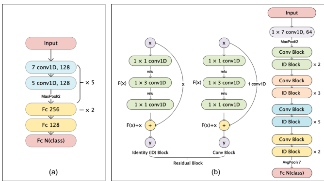
Figure 1. Proposed deep CNN architectures: (a) Baseline model; (b) ResNet-50-1D.
