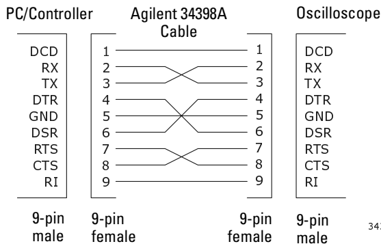
Pin out of Agilent 34398A RS-232 cable
