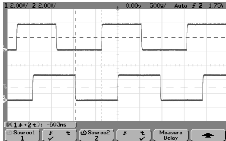
Delay Measurement
